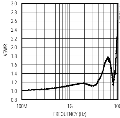
OUTPUT VSWR (DIFFERENTIAL)
